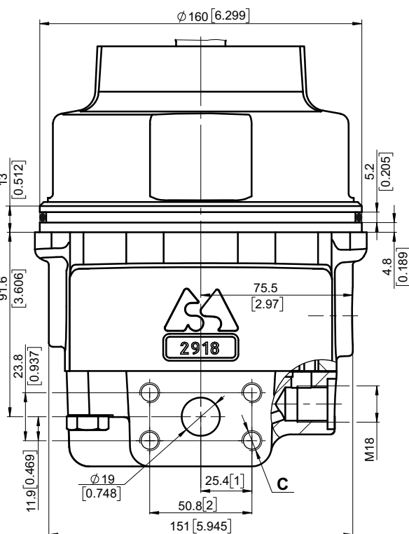
Side ports, port size default ,5and 9
